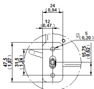
GIMBLE LOCK PLATE DETAIL
